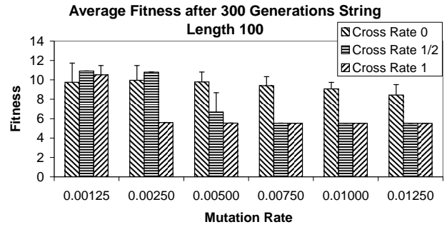
Figure 8: Average Fitness, \ell = 100 , k = 28 , 300 generations
